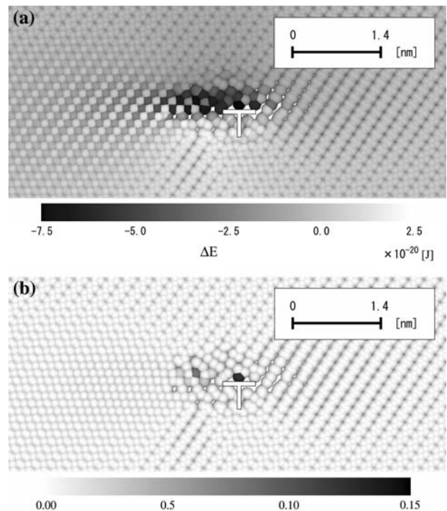
Fig. 2 (a) Distribution of potential-energy increment for each occupation site of hydrogen. (b) Probability of hydrogen occupation
