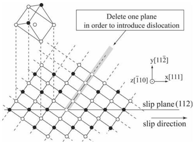
Fig. 1 Atomistic simulation model within an edge dislocation
